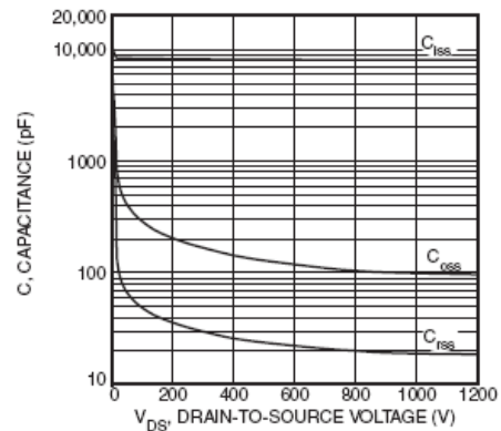
Figure 6, Capacitance vs. Drain-to-Source Voltage
