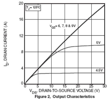
Figure 2, Output Characteristics
